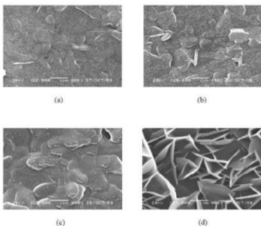
Fig. 2. SEM images of DR-1 films as deposited on ITO substrate for various electric fields (a) zero field, (b) E=0.59 MV/m, (c) E=1.9 MV/m, (d) E=3.3 MV/m.
