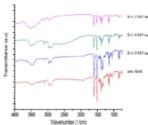
Fig. 4. FTIR spectrum of DR-1 films for various external electric fields
