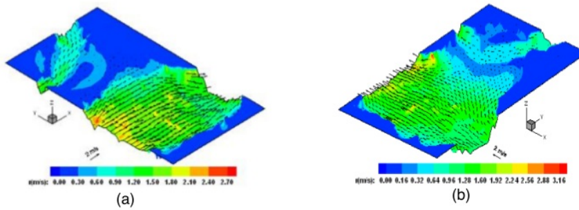
Figure 6. Simulated (3D) of marine current velocities distribution at seawater column of 20 m when low (a) and high (b) tide currents at 0.3 Sv
