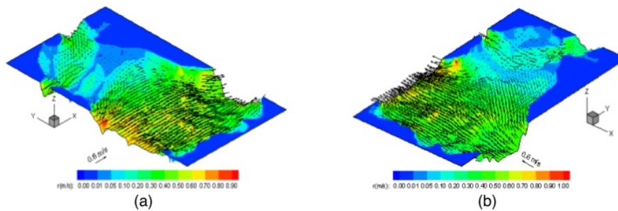
Figure 5. Simulated (3D) of marine current velocities distribution at seawater column of 20 m when low (a) and high (b) tide currents at 0.1 Sv
