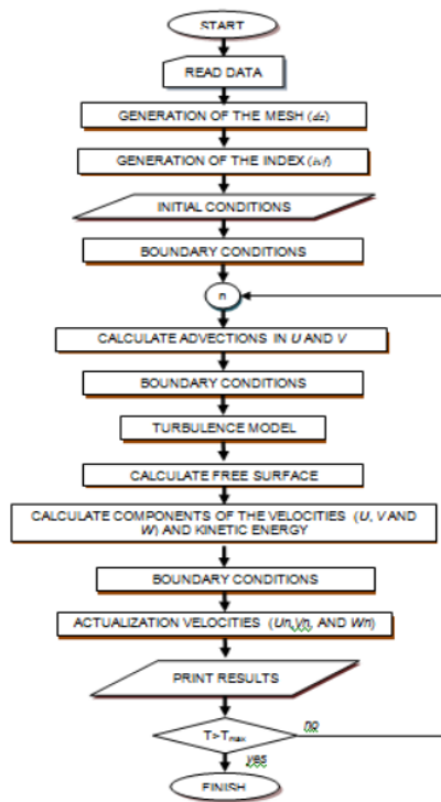
Figure 1. Flowchart of the numerical design
