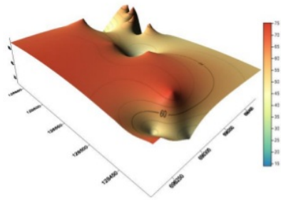
Figure 4. Geothermal Gradient Contour Map
