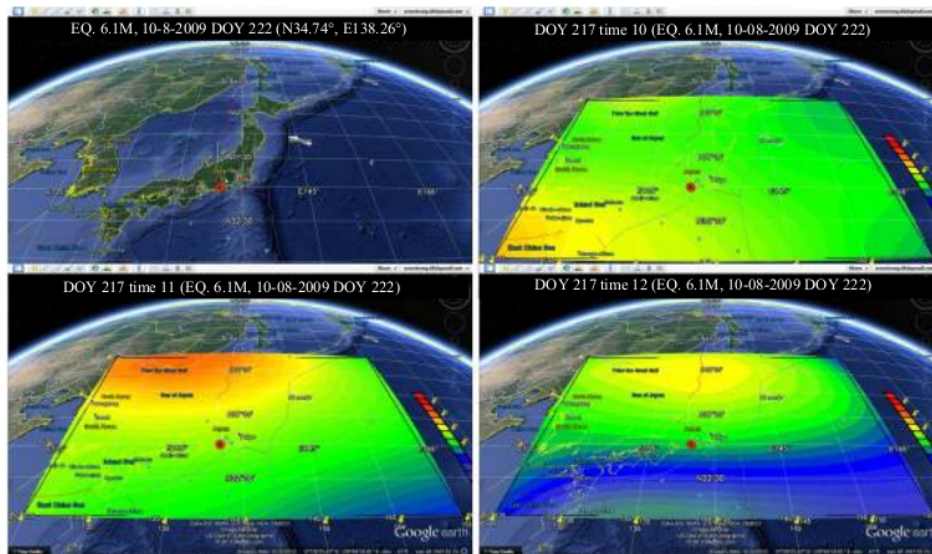
Fig. 4: GIM-TEC star model using Kriging Interpolation for M6.1 earthquake that occurred on August 10, 2009 show that the ionospheric precursors anomaly appeared 5 days before the earthquake precisely at 12.00 UT on August 05, 2009. From the anomaly, the position of the epicenter was visible point on the edge or outer portion of the anomaly
