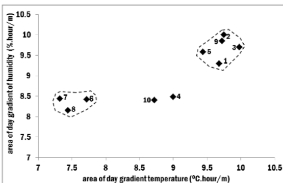
Fig.8: Transect grouping based on the area of gradient dynamic of temperature versus humidity at the day
