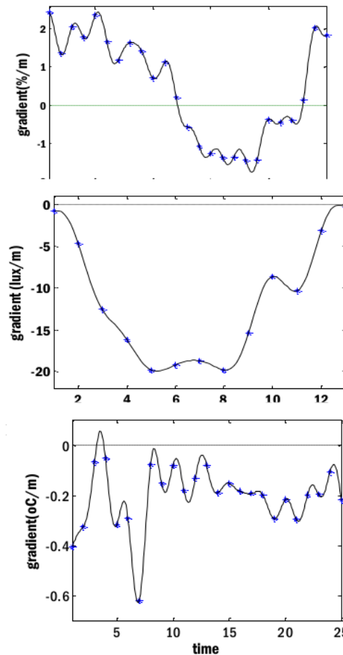
Fig.4: Graphic of water temperature gradient of transect-2 Talengen Bay
