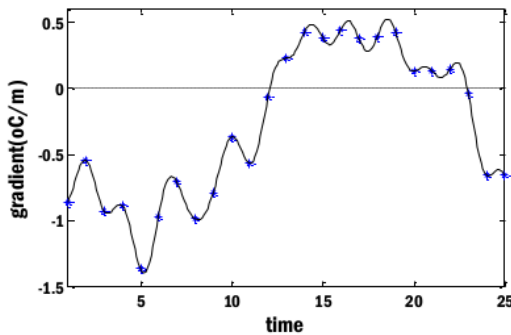
Fig.1: Graphic of air temperature gradient of transect-2, Talengen Bay
