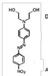
Figure 1. Molecular structure of Disperse Red-19
