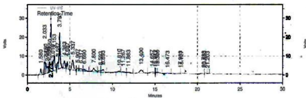
Retention time A1 (EtOH) extract
