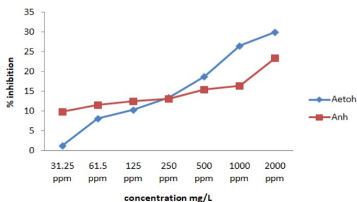
Figure 7. Extract inhibition activity at various test concentrations of DPPH free radicals
