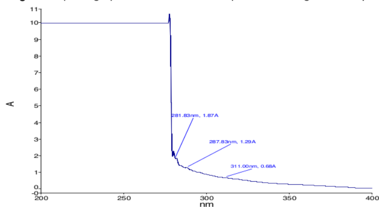
Figure 4. Spectrophotograph of n-hexan extract of Apis dorsata Binghami honey bee nest
