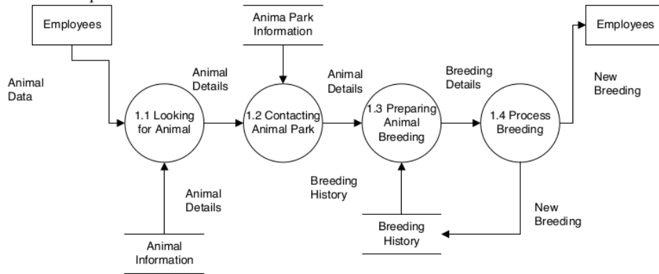
Figure 3. DFD Level 1
