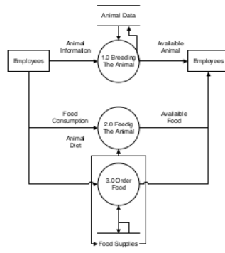
Figure 2. DFD Level 0
